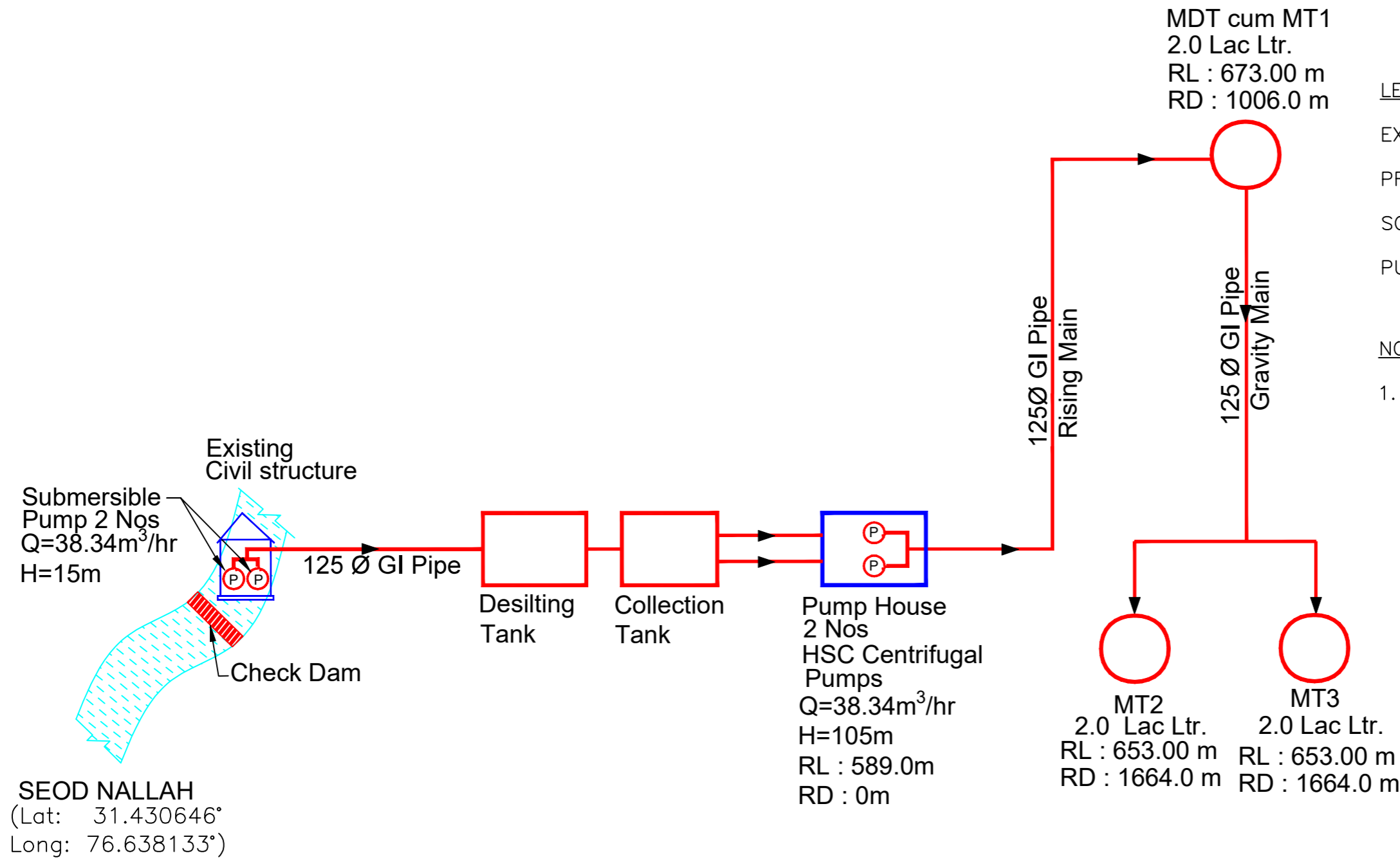
FLOW DIAGRAM OF PROPOSED LIS TIHRI (NON FUNCTIONAL SCHEME-29.15 Ha)
